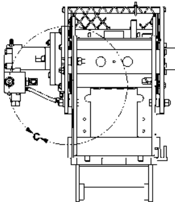
FRONT VIEW - SOME COMPONENTS REMOVED FOR CLARITY
