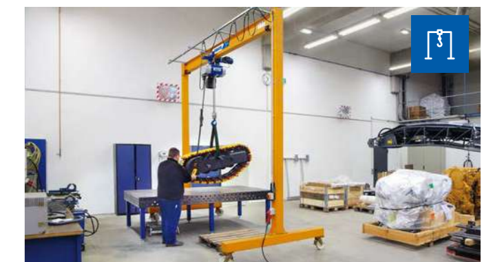
Lightweight mobile gantry LPK
